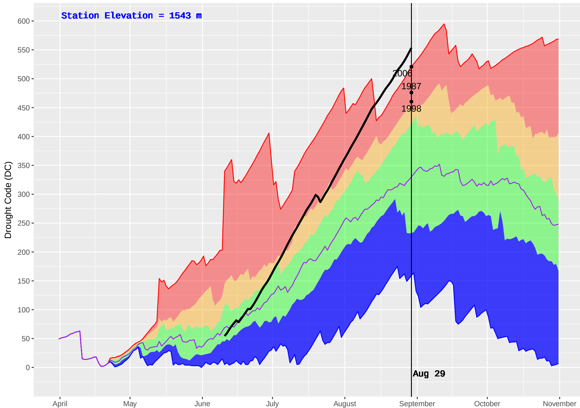
CAHILTY (253) : Historical (1987–2016) and Current (2017) Noon Drought Code (DC)
